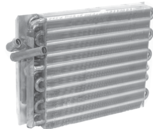
6901 10 3/4" x 10" x 2" In - 5/8" Out - 5/8" Volvo w/Bergstrom 108254; 176195
