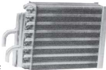
6902 8" x 9" x 2 1/2" In - 5/8" Out - 5/8" Western Star 4800-4900 RD10460-1
