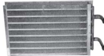
6897 8" x 18 11/16" x 1 7/8" In - 5/8" Out - 5/8" Peterbilt 108289, MC1365
