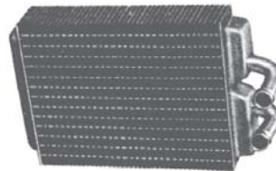
6845 6" x 7 3/4" x 2" In - 5/8" Out - 5/8" Ford C, CL, CLT, CT E6HZ-18476B
