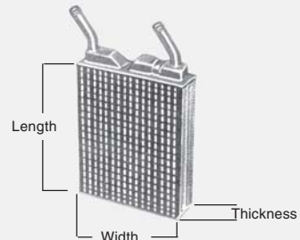
6901 10 3/4" x 10" x 2" In - 5/8" Out - 5/8" Volvo w/Bergstrom 108254; 176195
