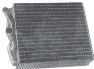
6838 7 1/2" x 8 1/4" x 2" In - 5/8" Out - 3/4" Che/GMC Bison/General 3033461
