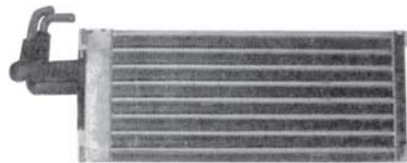
6903 8" x 17 1/2" x 1 7/8" In - 5/8" Out - 5/8" Freightliner FL Series 315060; BOA85-200-71-009
