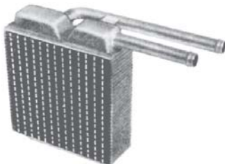
6835 6" x 6" x 2" In - 5/8" Out - 5/8" Ford 73-79 F150/350 D2TZ-18476C
