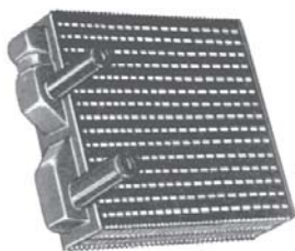
6829 7" x 8 1/4" x 2" In - 5/8" Out - 3/4" Che/GMC P30, 3027247
